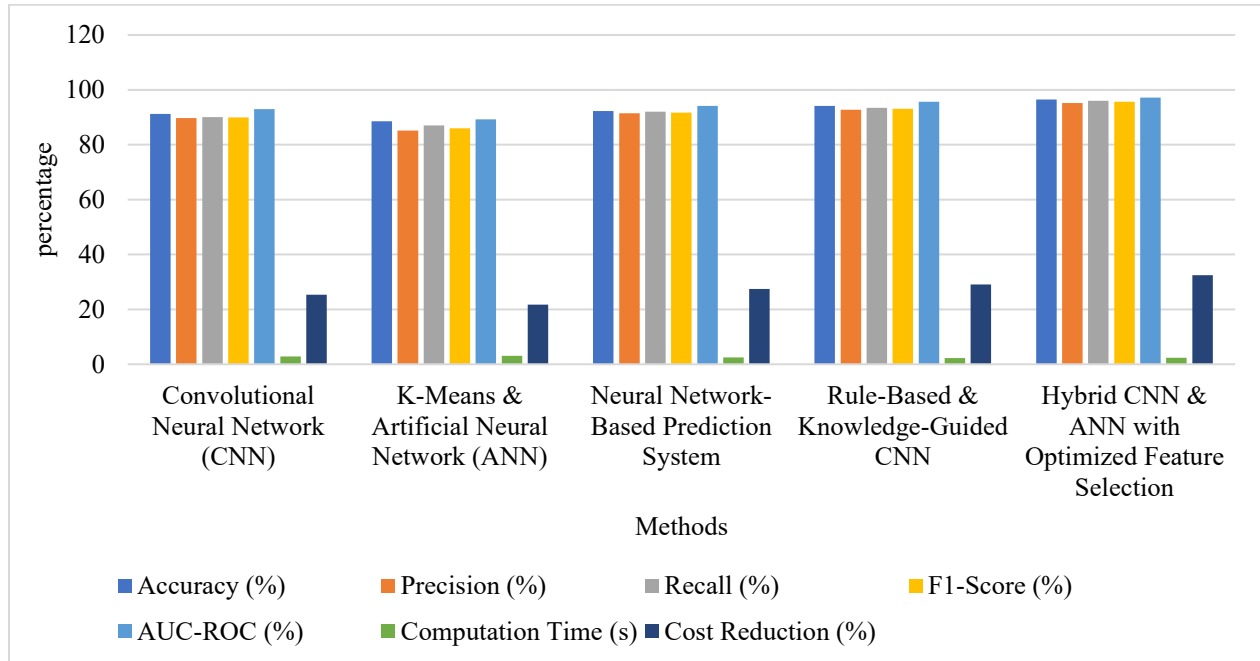
Figure 3: Performance Comparison of AI Models: Accuracy, Precision, and Computational Efficiency
