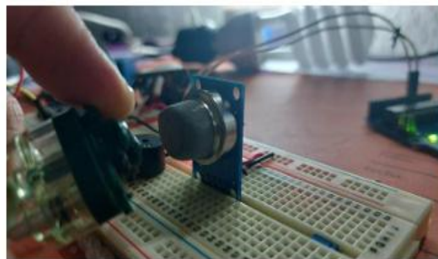
Fig. F.- The gas sensor is stimulated by means of a igniter to verify that the host is receiving the information and displaying it correctly..
