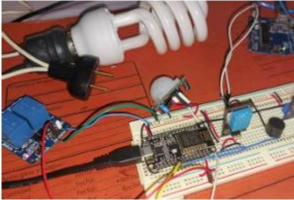
Fig. N.- Final physical representation of the final circuit controlled through the NodeMCU, already using voice commands.
